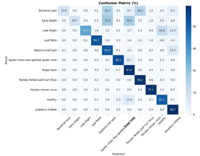
GAMBAR II. CONFUSION MATRIX (%)
